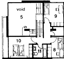
upper floor
